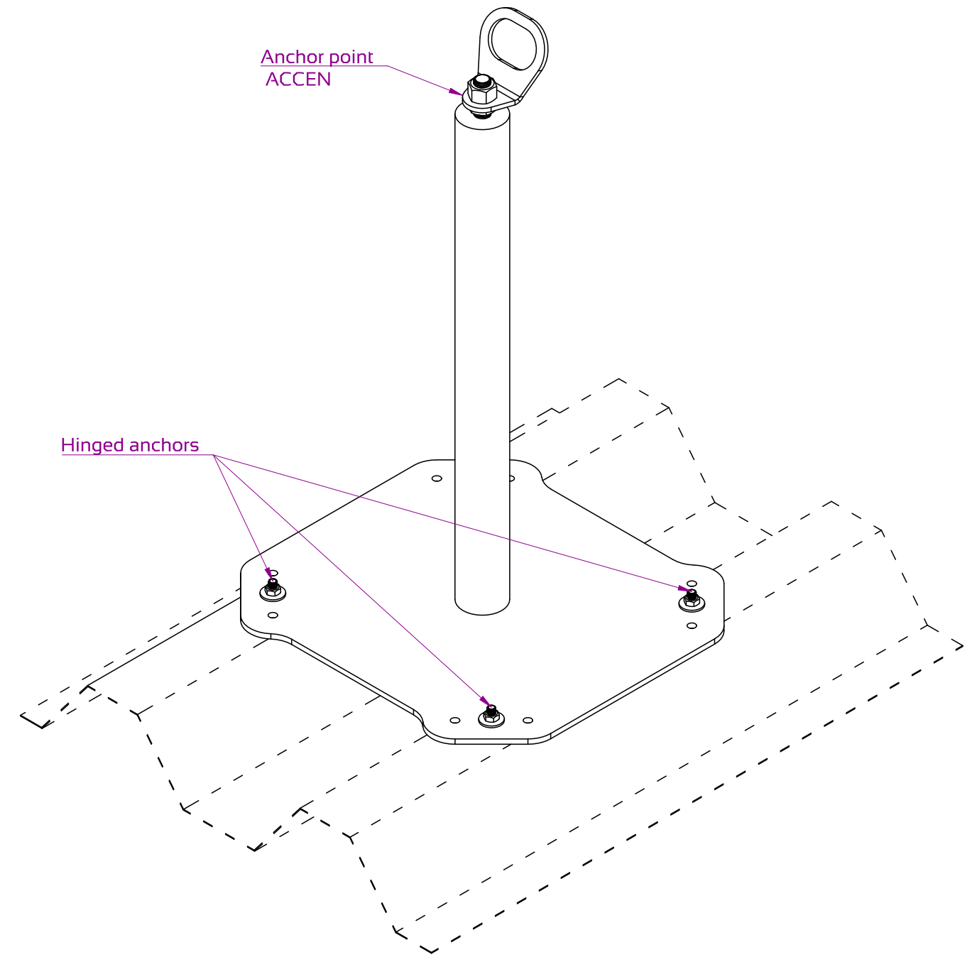
Isometric view scale 1:5
