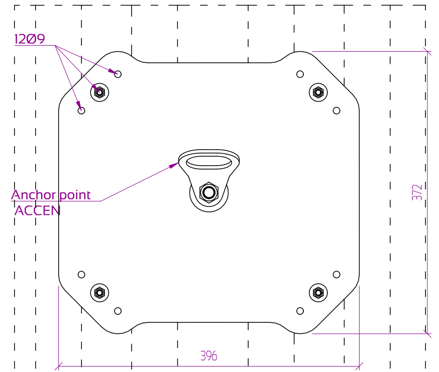
View WI scale 1:5
