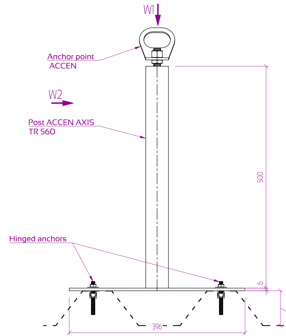
Post ACCEN AXIS TR 560 scale 1:5
